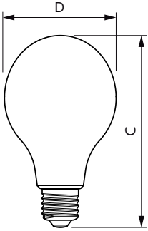
Bulb A23 110-130V 5-W lm K E27 ND
