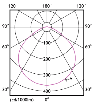
LEDTForce HB 140W Others E40 120D
