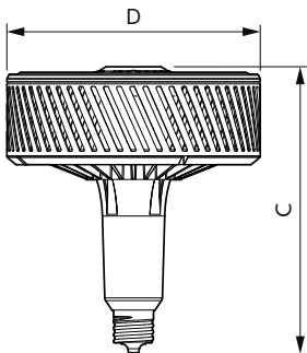
TForce HB MV ND 200-140W E40 840 WB
